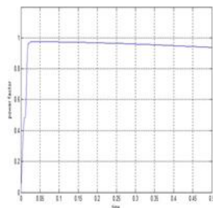
Figure.13 Power factor for current source inverter.
