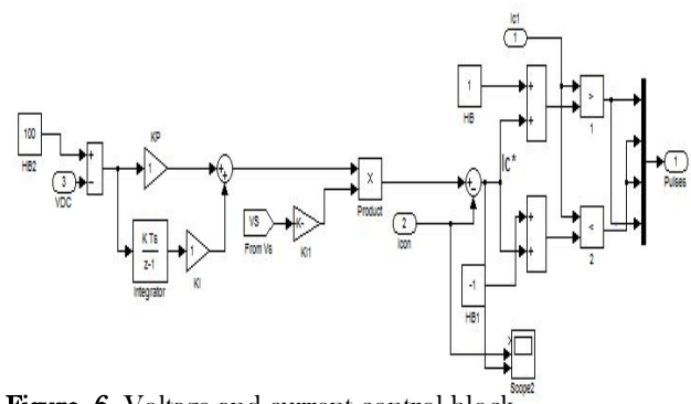
Figure. 6. Voltage and current control block.
