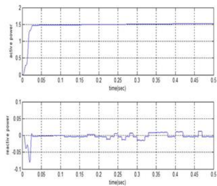
Figure. 14. Active and reactive power wave forms of zsi inverter.
