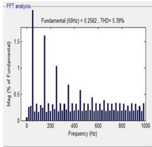
Figure. 17. Total harmonic distortion for csi system. The above (Figure 16) and (Figure 17) presents the total harmonic distortion of ZSI and CSI respectively. From this we can conclude that THD of ZSI value 1.67 is improved than the CSI value 5.39.
