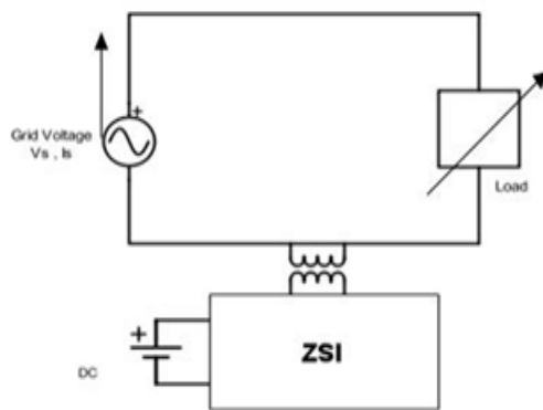
Figure.1 Z-source inverter topology
