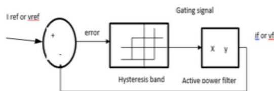
Figure.4 Hysteresis control technique
