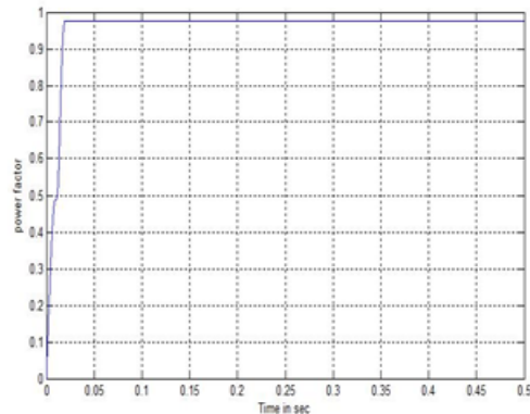
Figure. 12. Power factor for proposed zsi system.
