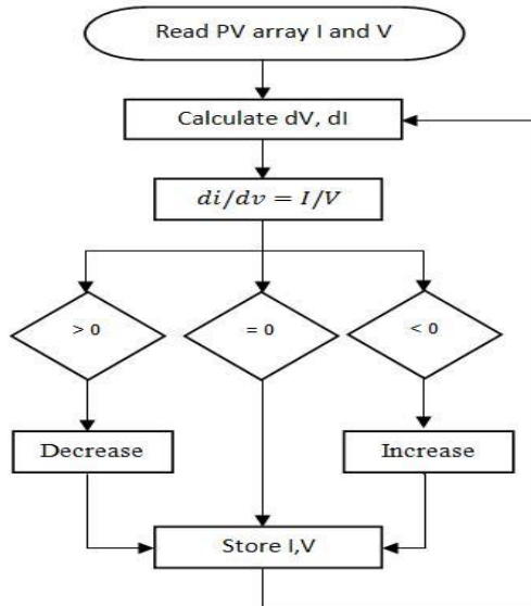
Figure.3 Incremental conduction algorithm. IV. Hysteresis Current Control Method
