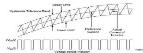
Figure. 5 Hysteresis band V. Proposed System Control Technique
