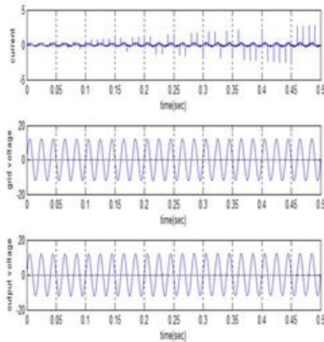
Figure.11. Current and voltage waveforms for CSI system.
