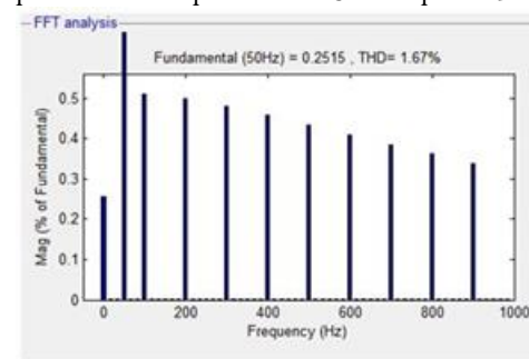
Figure. 16. Total harmonic distortion for proposed ZSI system.
